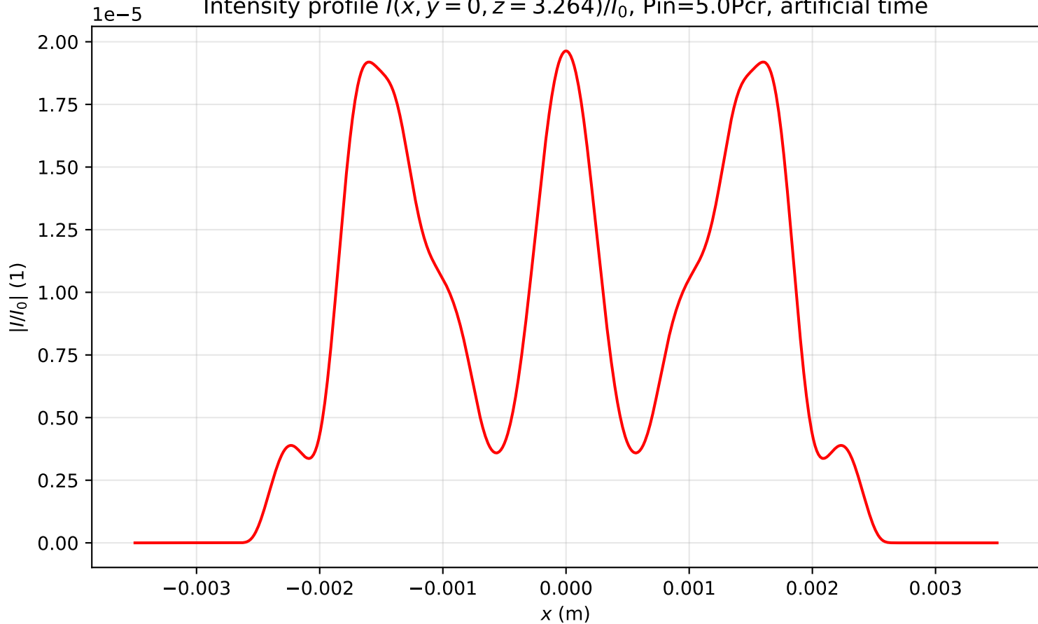
Intensity profile I(x, y = 0, z = 3.264)/I_0 , P_{in}=5.0P_{cr} , artificial time
